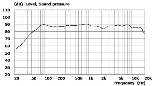
Frequency Response
