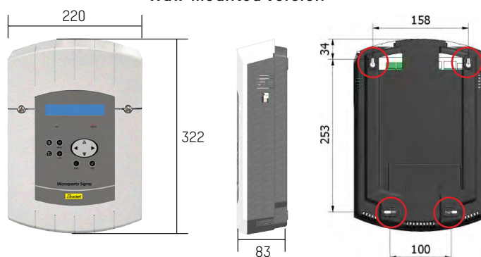
Wall-mounted version
